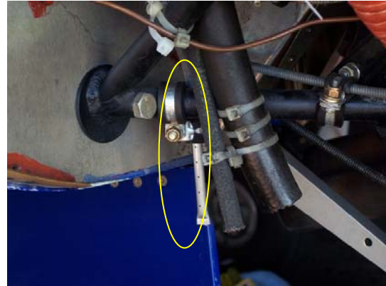
Figure 6, Piccolo tube at cowl exit
