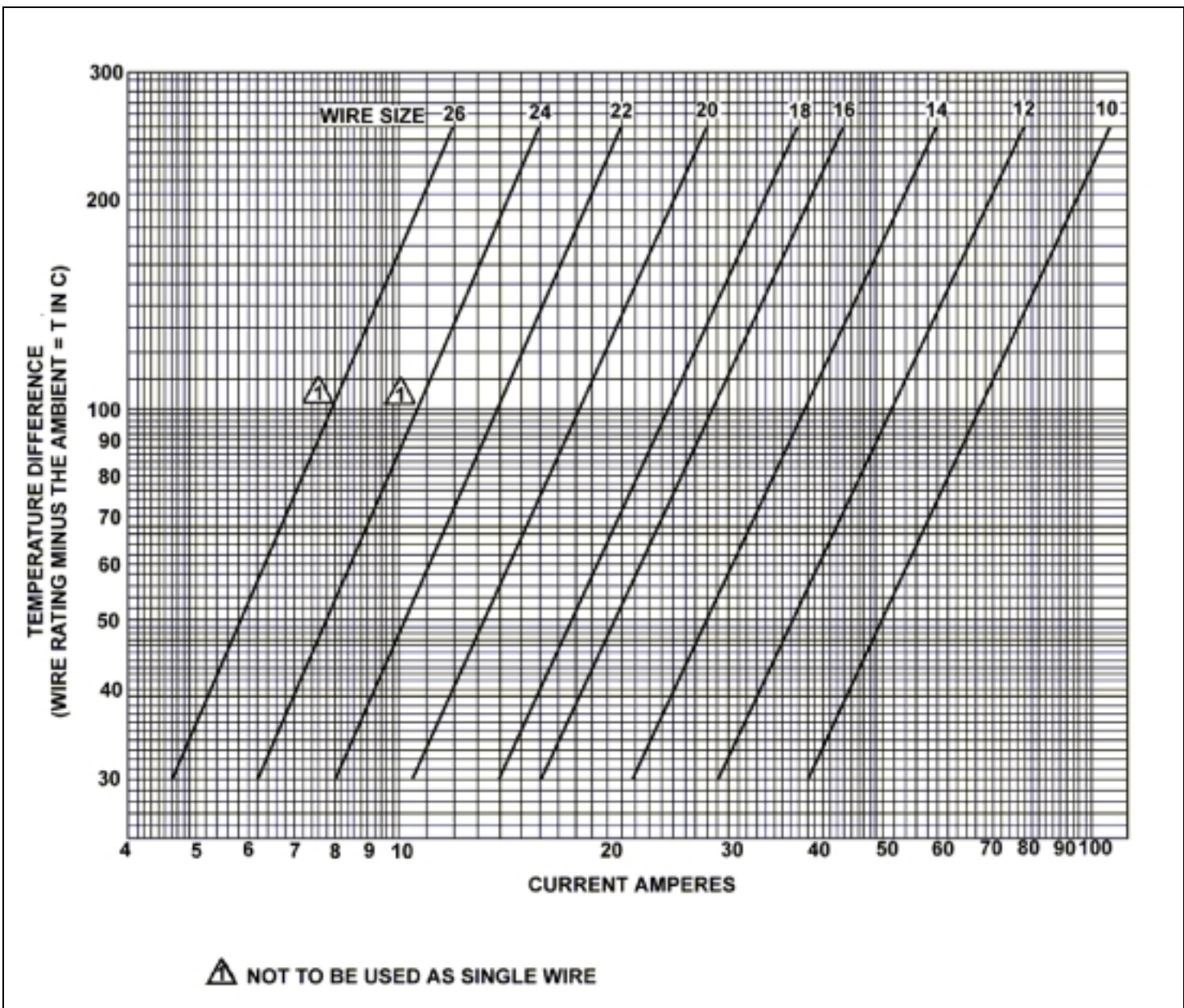
FIGURE 11-4a. Single copper wire in free air.
