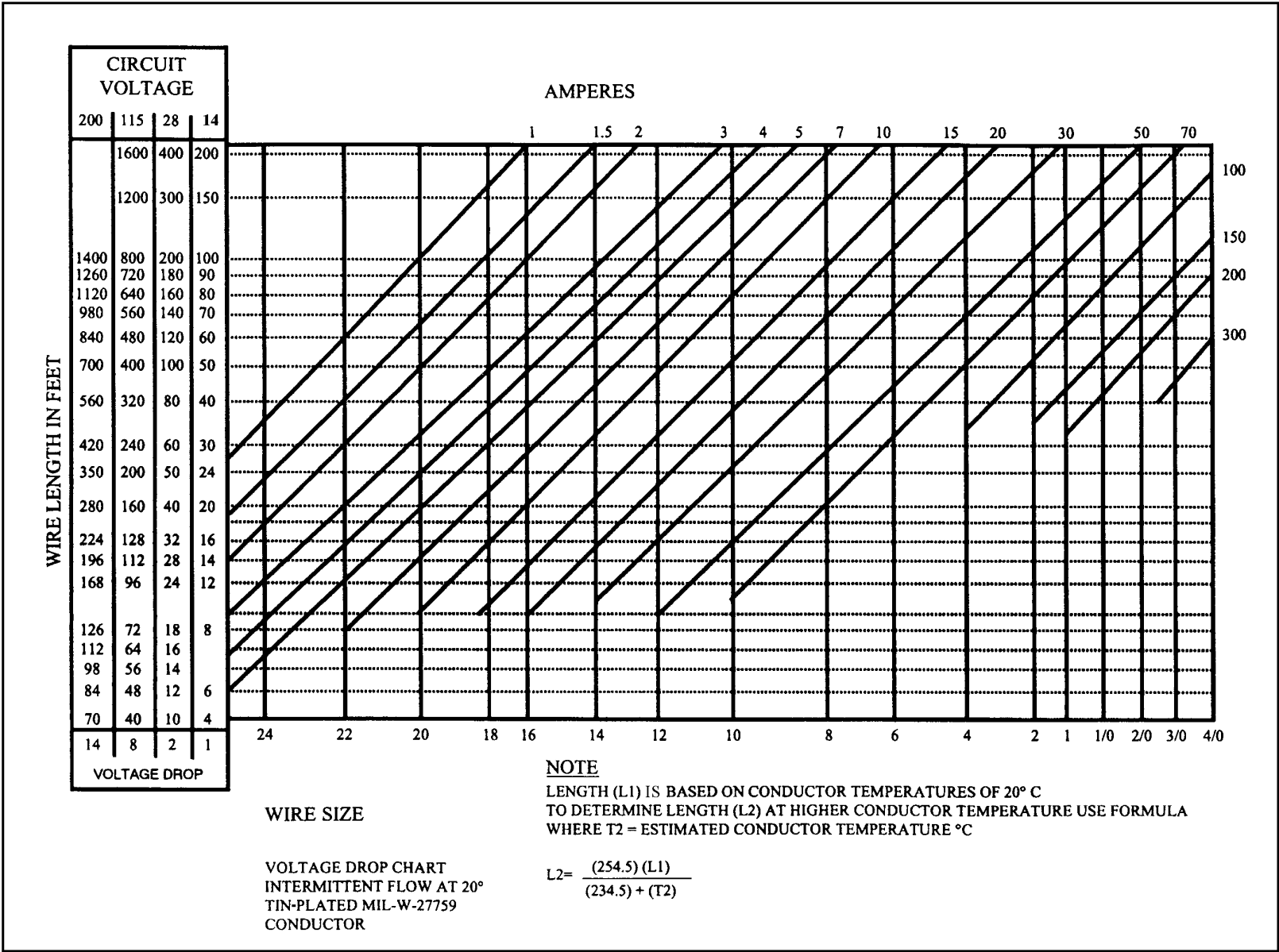
FIGURE 11-3. Conductor chart, intermittent flow.
