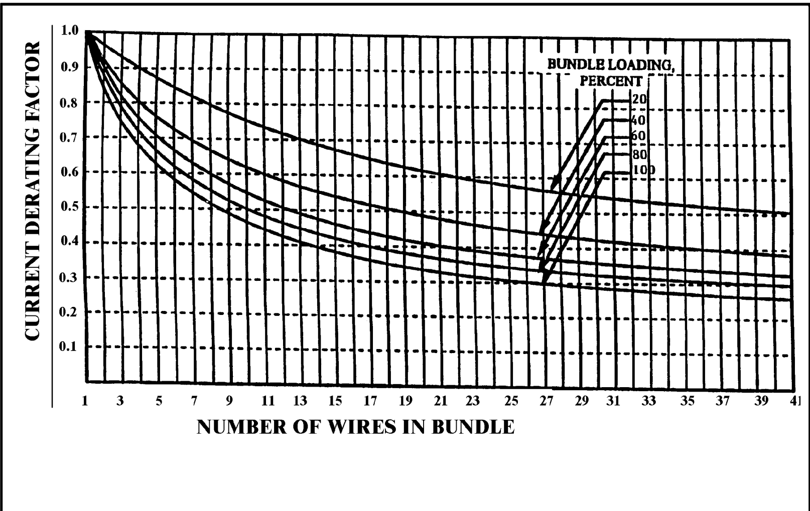
FIGURE II-5. Bundle derating curves.
