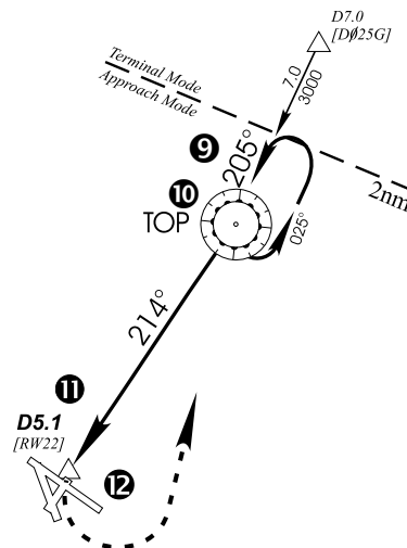
Figure 6-44 Approach Mode
