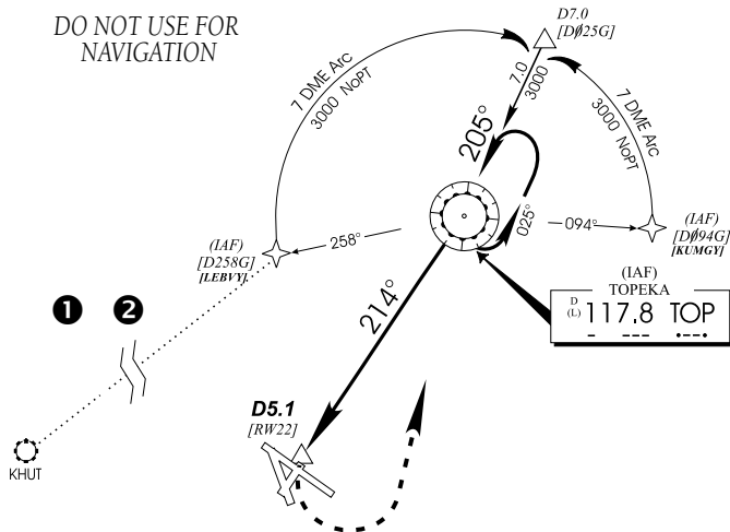
Figure 6-36 Enroute Mode
