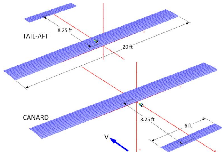
Figure C2-12: The two VL models. The conventional configuration is to the left and canard to the right.
