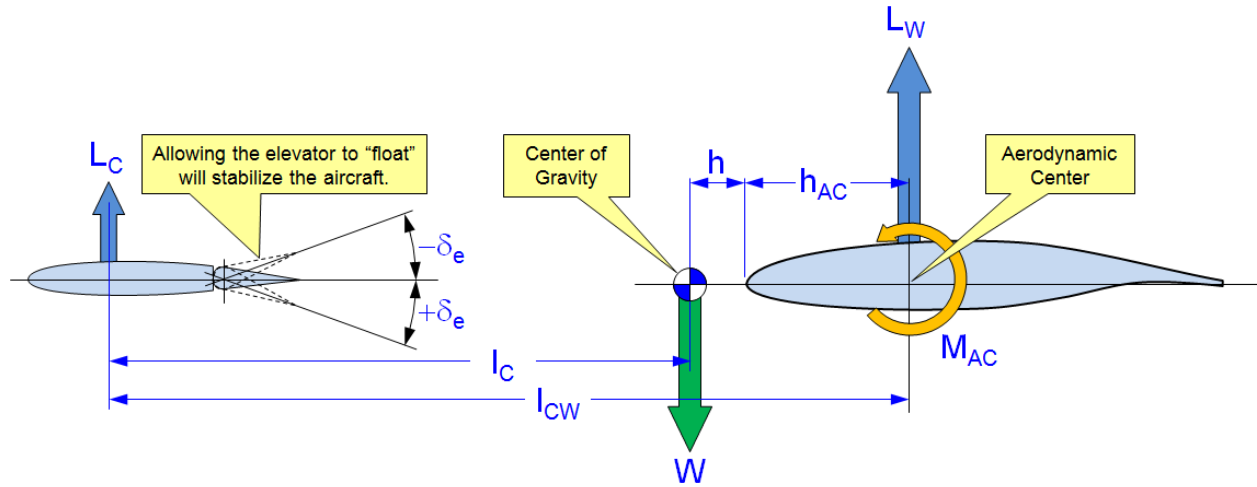
Figure C2-4: Wing-Canard system used to derive Equation (C2-4).
