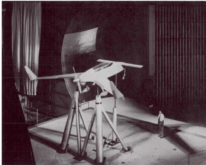
Figure C2-9: An image from Reference 2, showing the Rutan VariEze mounted in the wind tunnel at the LFST.
