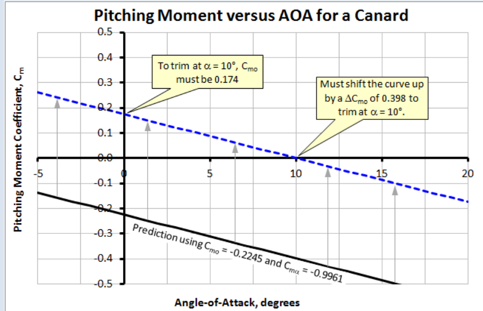
Figure C2-5: The pitching moment coefficient calculated for the arbitrary value of h = 0.783 ft (solid curve). The dashed curve represents how the solid curve must be shifted to allow the vehicle to be trimmed at a \alpha = 10^\circ . The upward shift can be accomplished by deflecting the elevator TED or using a cambered airfoil (or a combination thereof).
