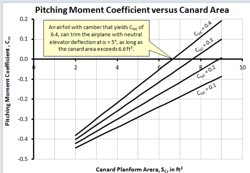
Figure C2-8: The pitching moment coefficient plotted in terms of the canard planform area, constant l_C = 8.25 \text{ ft} , and considering four airfoil options. This reveals that the example aircraft will also need a highly cambered airfoil to keep the size of the canard down. Note that SM = 0.10 and \alpha = 5^\circ .
