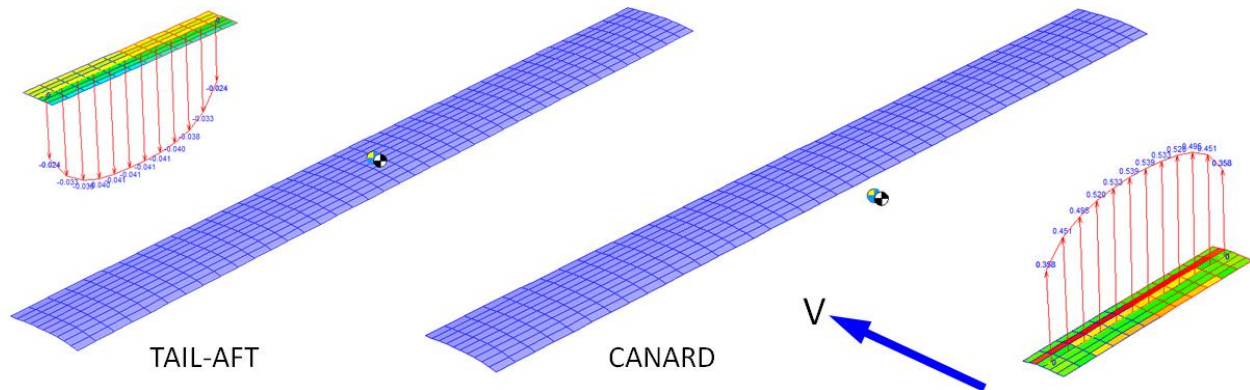
Figure C2-17: Distribution of section lift coefficients on the stabilizing surfaces.
