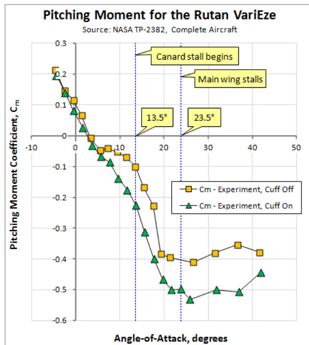
Figure C2-11: The pitching moment for the Rutan VariEze with and without leading edge droops (cuffs). (Reproduced from Reference 2)
