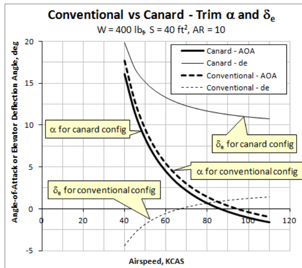
Figure C2-15: Comparing AOA and elevator deflection required to trim the conventional and canard configurations at the given airspeed.
