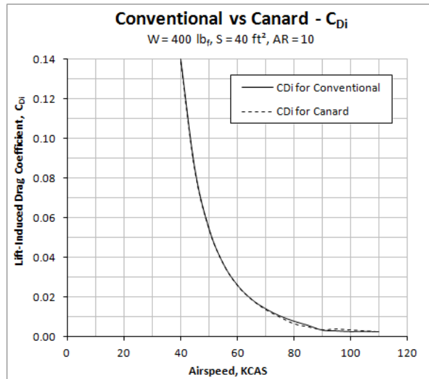
Figure C2-14: Comparing lift-induced drag of the conventional and canard configurations.
