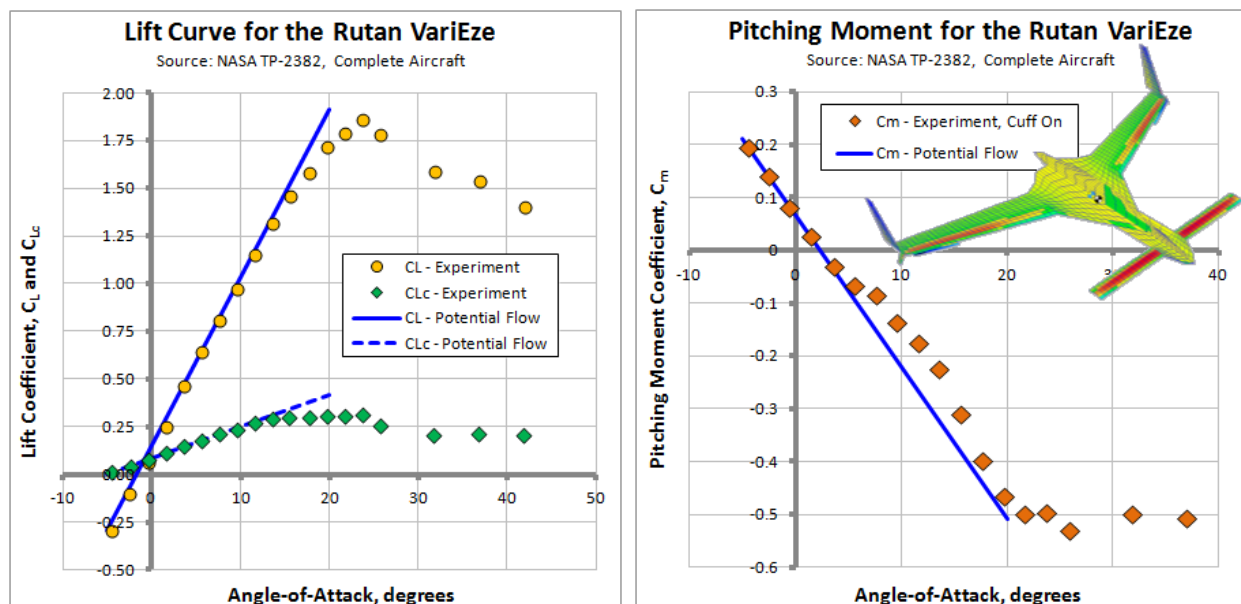
Figure C2-13: Comparing lift and pitching moment of a validation model to experiment.
