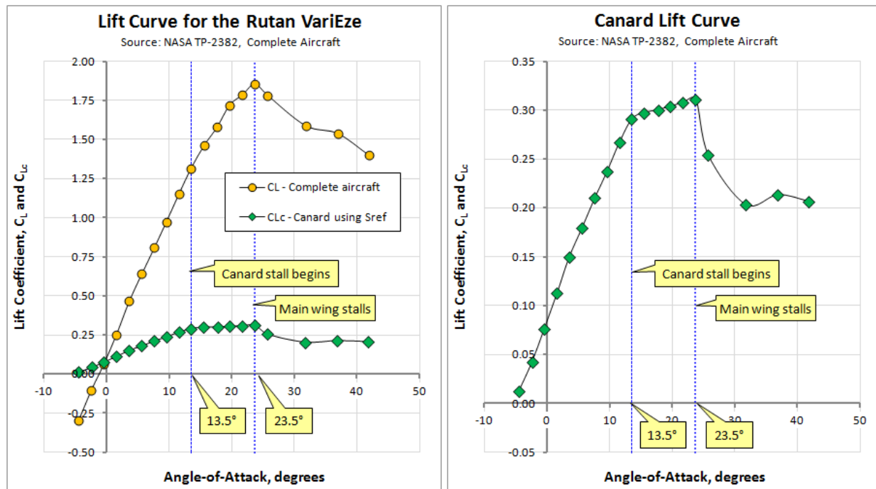
Figure C2-10: The lift curves for the entire aircraft and the canard. The right graph shows the lift curve of the canard in detail. (Reproduced from Reference 2)
