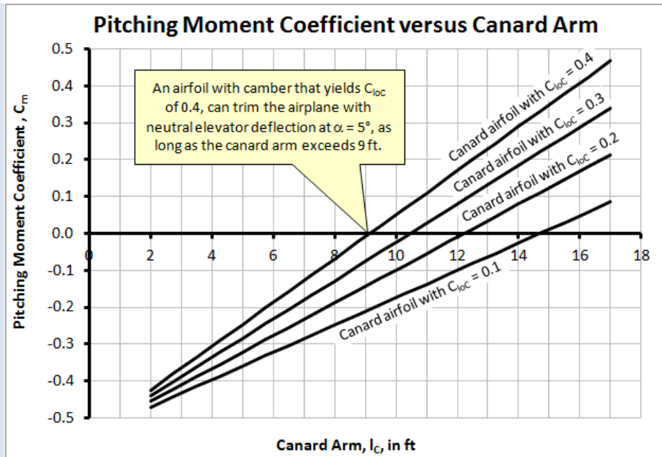
Figure C2-7: The pitching moment coefficient plotted in terms of the canard arm, constant S_C = 6 \text{ ft}^2 , and considering four airfoil options. This reveals that the example aircraft will need a highly cambered airfoil if the goal is to keep the length of the fuselage down. Note that SM = 0.10 and \alpha = 5^\circ .
