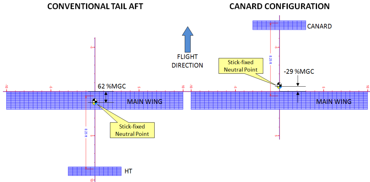
Figure C2-3: Comparing the stick-fixed neutral points and CG locations required for a Static Margin of 0.10 of a conventional tail aft (left) and canard (right) configurations. The neutral points were determined using potential flow theory. Note the numbers only apply to this specific geometry.
