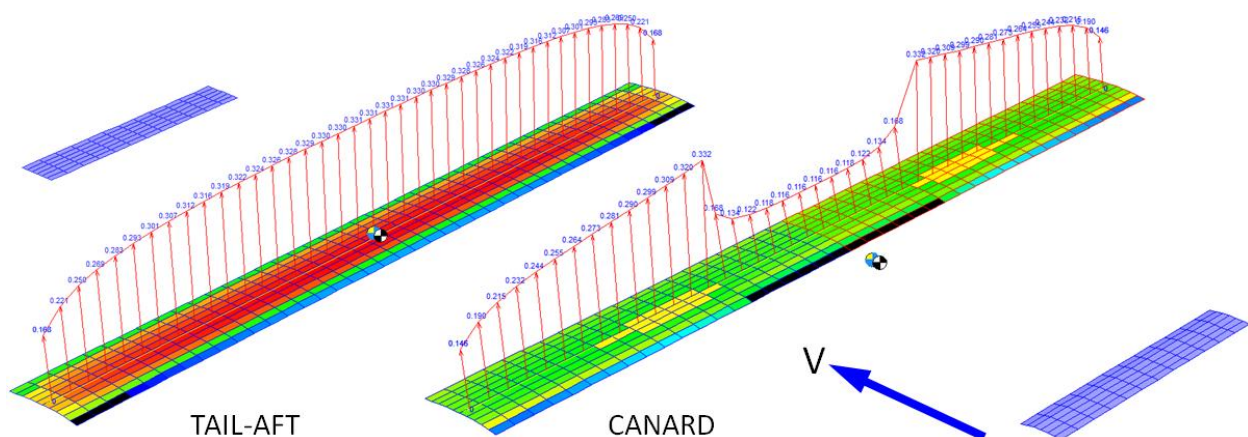
Figure C2-16: Distribution of section lift coefficients on the wing.
